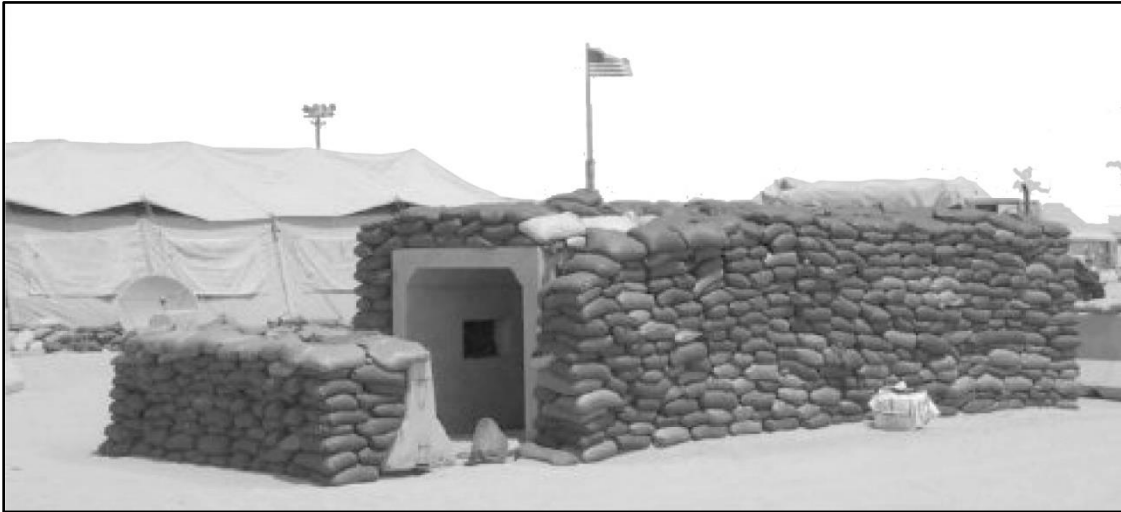
Figure 5-13. Properly sandbagged concrete shelter
