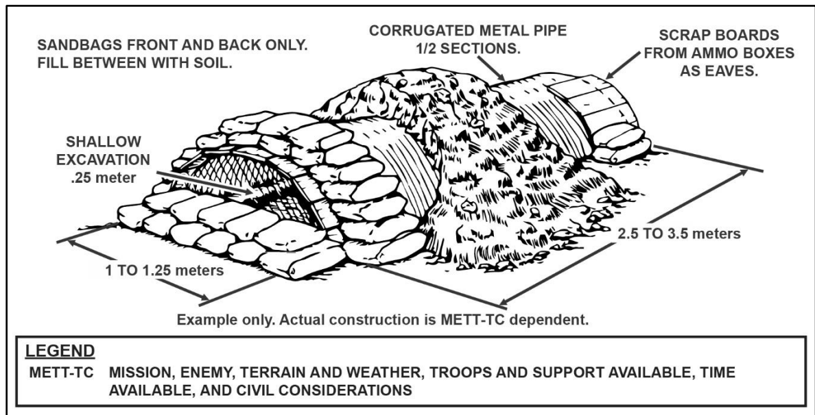
Figure 5-7. Example of fighting position with corrugated metal culvert halves
