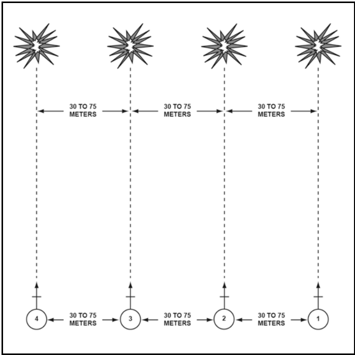
Figure 2-11. Parallel sheaf
