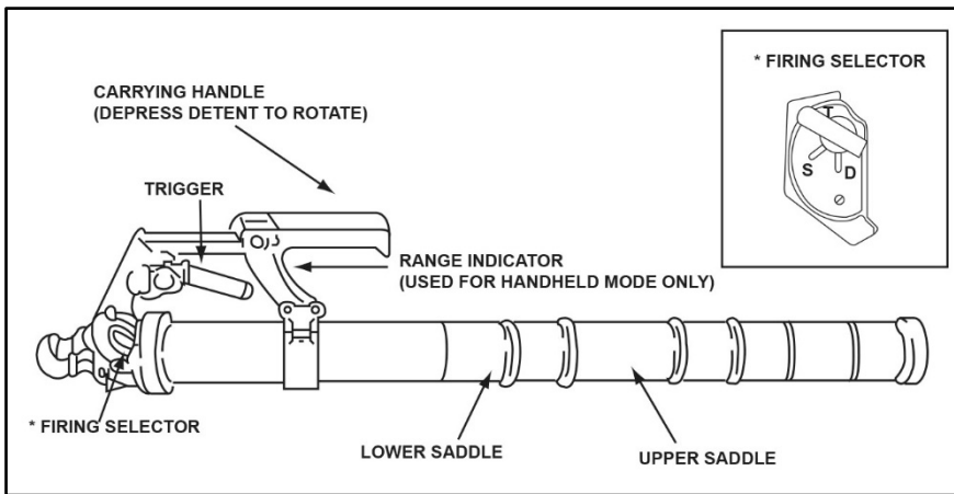
Figure 3-2. M225/M225A1 cannon assembly
