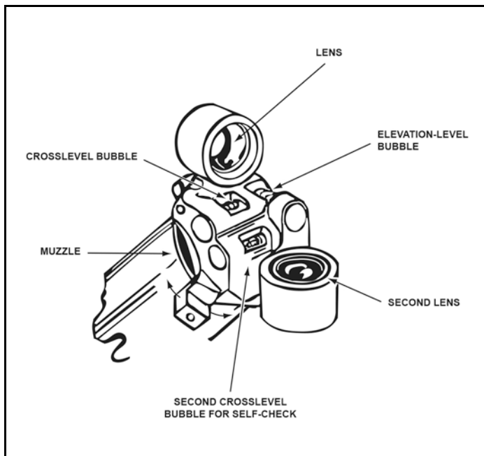
Figure 2-2. M115 boresight
