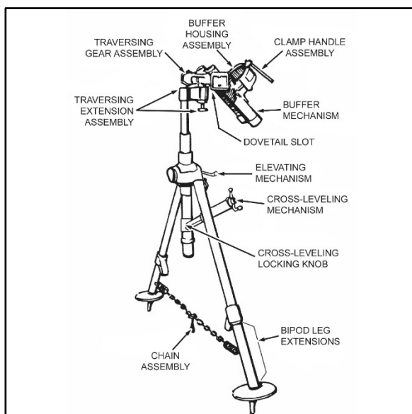
Figure 5-4. M191 bipod assembly (carrier- or ground-mounted)
