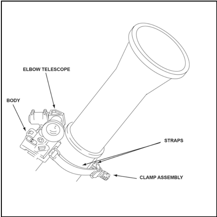
Figure 2-1. M45 boresight
