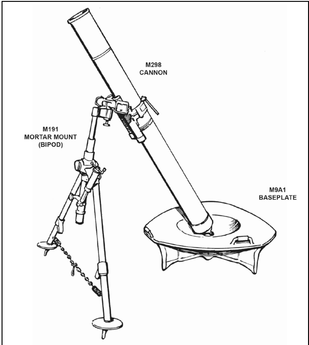
Figure 5-2. 120-mm mortar
