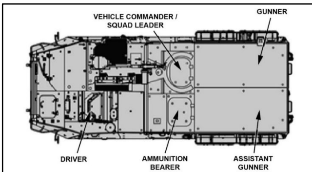
Figure 5-27. Squad configuration
