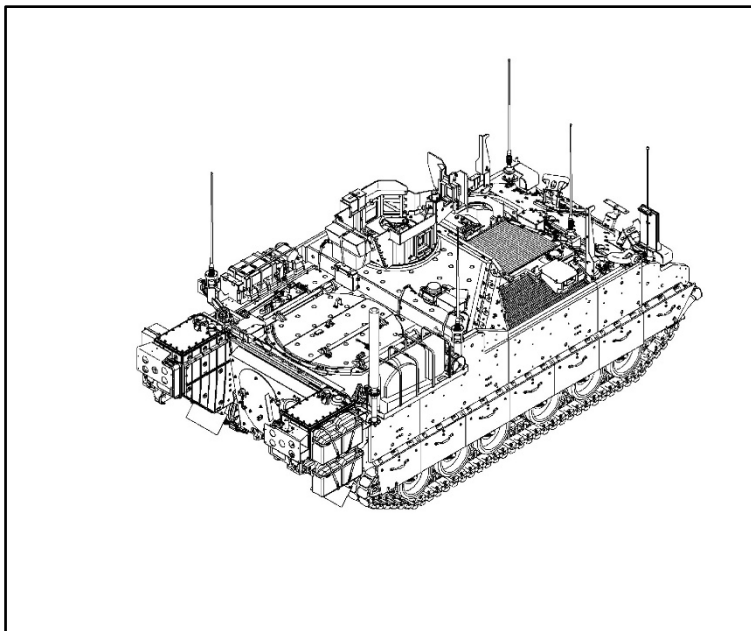
Figure 5-24B. XM1287 mortar carrier, right rear view
