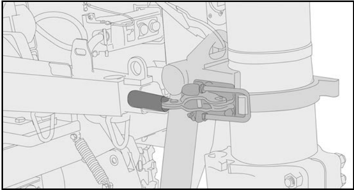
Figure 5-16B. Tube clamp
