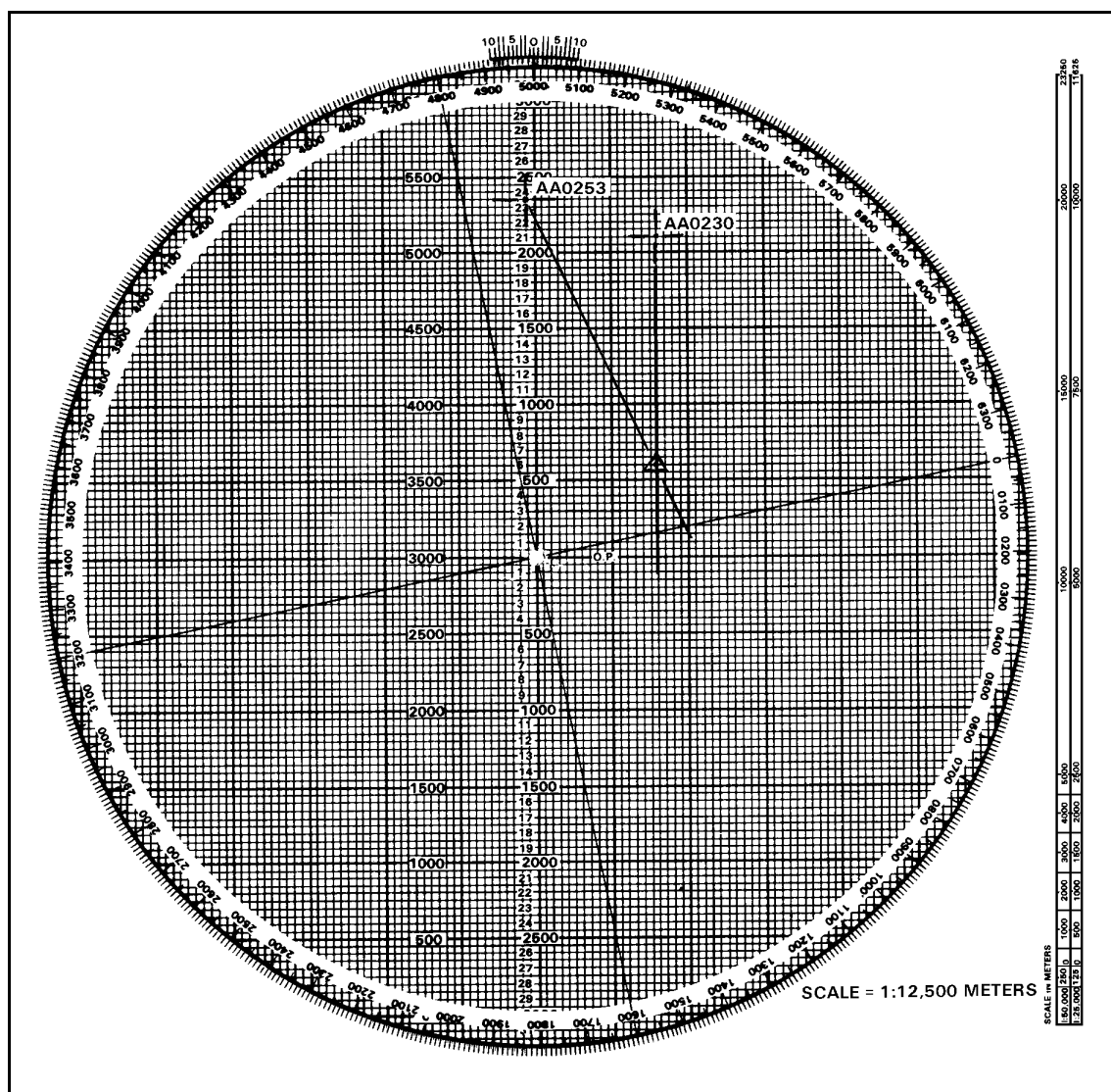
Figure 12-23. Resection.
