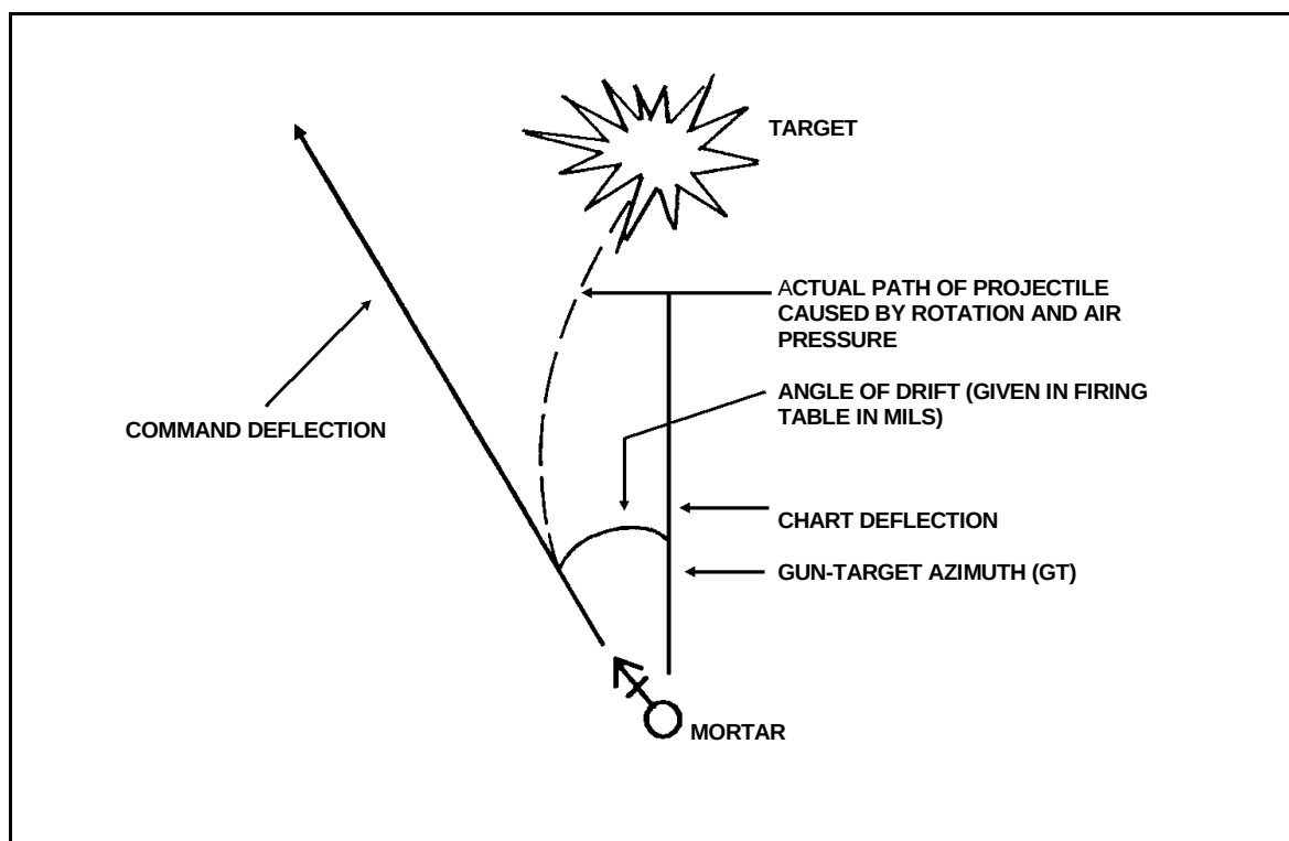
Figure 2-3. Drift.
